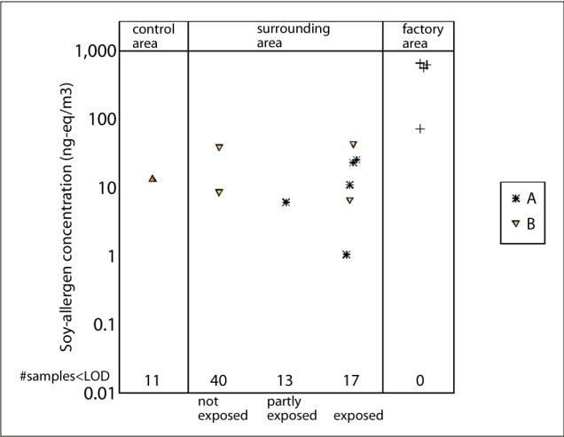
Figure 1. Soy allergen concentrations in control area, area surrounding the factory and outside on factory premises. A – sampling location north of factory. B – sampling location southeast of factory in the vicinity of soy scrap transport route. The number of samples with undetectable soy allergen concentrations are shown (# samples<limit of detection)
