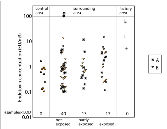
Figure 2. Endotoxin concentrations in control area, area surrounding the factory and outside on factory premises. A – sampling location north of the factory. B – sampling location southeast of factory in the vicinity of soy scrap transport route. The number of samples with undetectable endotoxin concentrations are shown (# samples<limit of detection)
