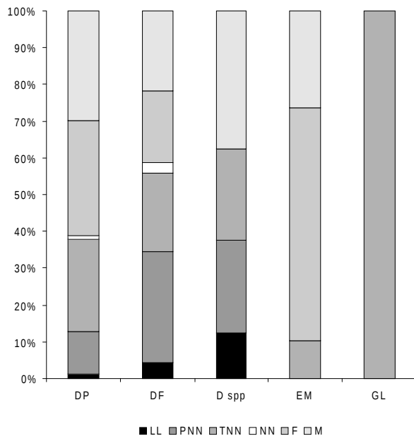
Figure 4. Age structure of populations of pyroglyphid dust mite species in a total of dust samples from the examined dwellings. Key: DP - Dermatophagoides pteronyssinus ; DF - D. farinae ; D spp - Dermatophagoides spp.; EM - Euroglyphus maynei ; GL - Gymnoglyphus longior ; LL - larvae; PNN - protonymphs; TNN - tritonymphs; NN - nymphs unidentified; F - females; M - males.
