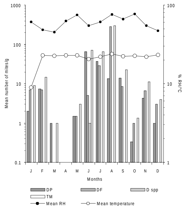
Figure 3. Annual dynamics of pyroglyphid mite species (mean number of mites per 1 gram of dust) in pooled floor/carpet dust samples from examined dwellings and mean values of relative humidity and temperature. Key: DP - Dermatophagoides pteronyssinus ; DF - D. farinae ; D spp - Dermatophagoides spp.; TM - total mites; RH - relative humidity.
