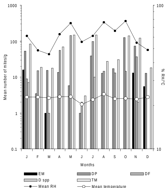
Figure 1. Annual dynamics of pyroglyphid mite species (mean number of mites per 1 gram of dust) in pooled bed/mattress dust samples from examined dwellings and mean values of relative humidity and temperature. Key: EM - Euroglyphus maynei ; DP - Dermatophagoides pteronyssinus ; DF - D. farinae ; D spp - Dermatophagoides spp.; TM -total mites; RH - relative humidity.
