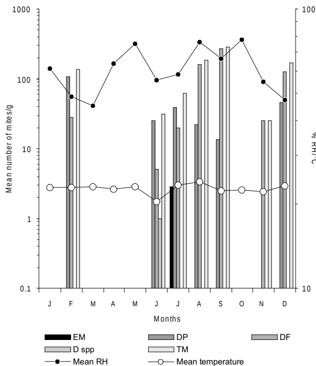
Figure 2. Annual dynamics of pyroglyphid mite species (mean number of mites per 1 gram of dust) in pooled dust samples from upholstery furniture in examined dwellings and mean values of relative humidity and temperature. Key: EM - Euroglyphus maynei ; DP - Dermatophagoides pteronyssinus ; DF - D. farinae ; D spp - Dermatophagoides spp.; TM - total mites; RH - relative humidity.
