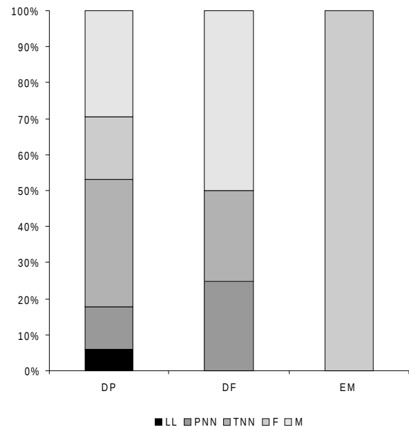
Figure 5. Age structure of populations of pyroglyphid dust mite species in a total of dust samples from the examined hospitals. Key: DP - Dermatophagoides pteronyssinus ; DF - D. farinae ; EM - Euroglyphus maynei ; LL - larvae; PNN - protonymphs; TNN - tritonymphs; F - females; M - males.
