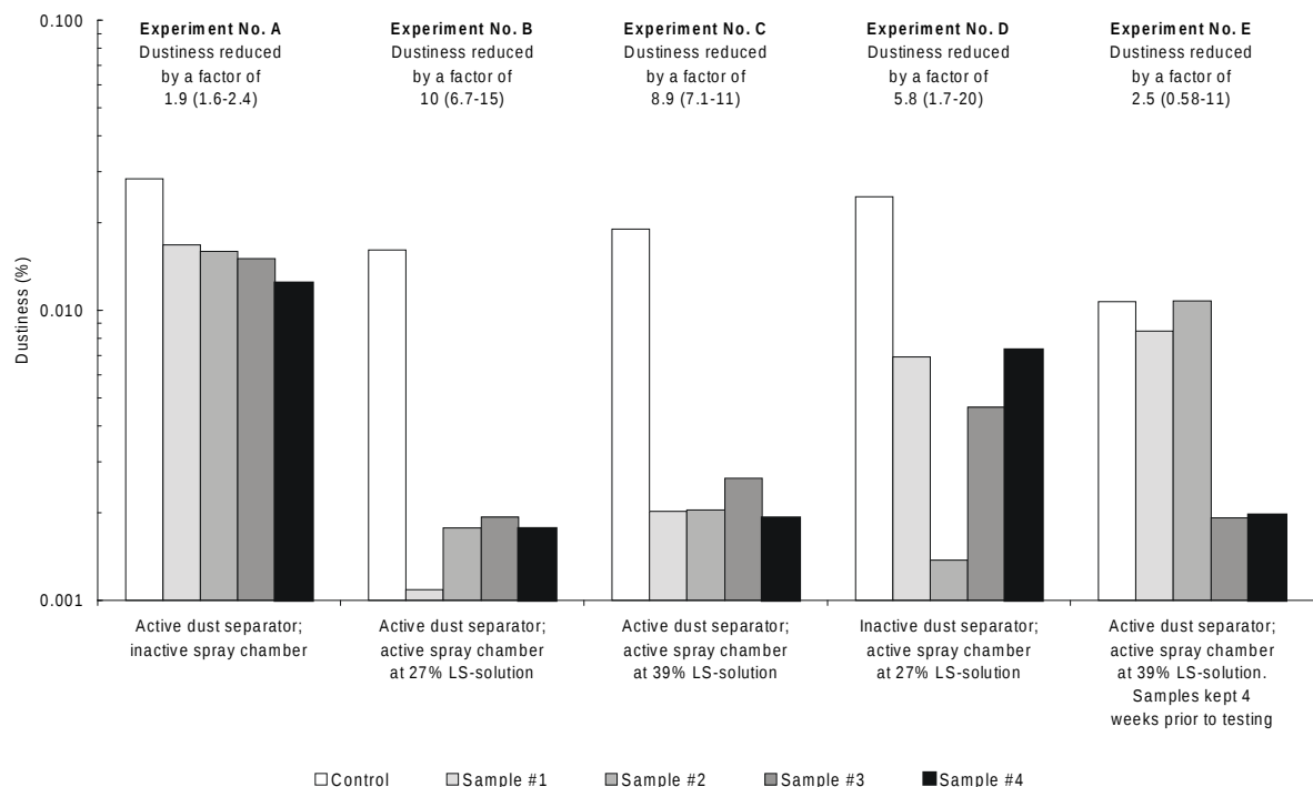
Figure 3. Dustiness (%) of chopped straw (barley) versus different techniques to reduce the dustiness. The factor of reduction in dustiness is given with reference to the control sample and is presented as the geometric mean and the 95% confidence interval in parentheses.
