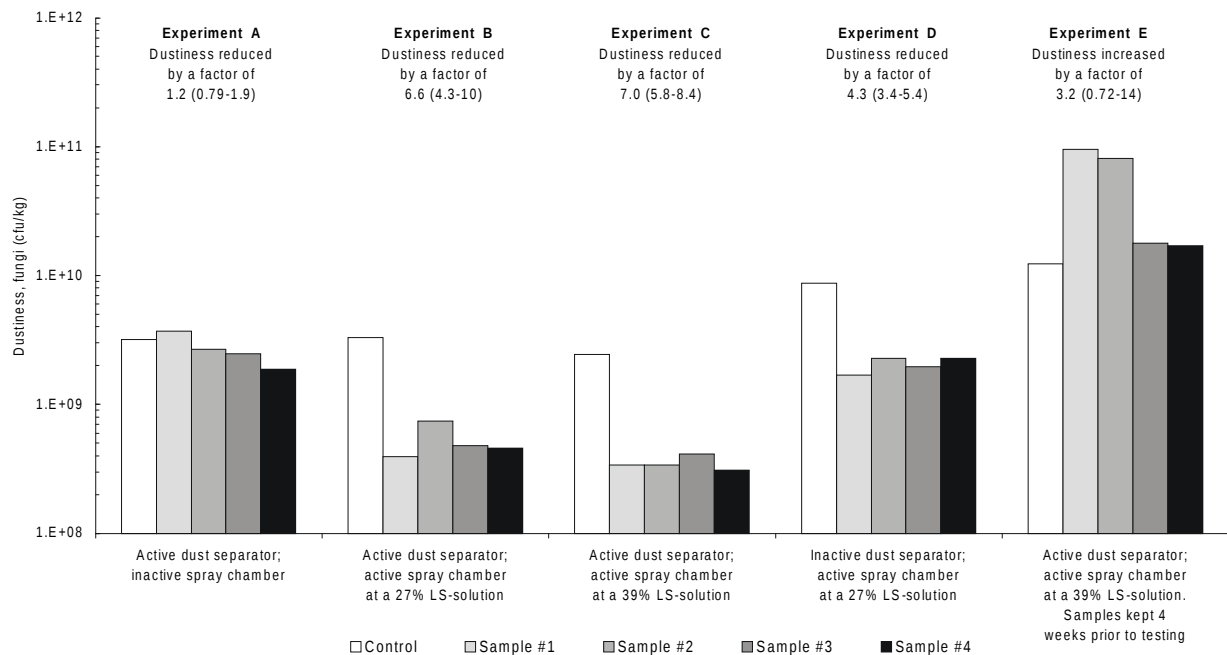
Figure 5. Dustiness of chopped straw (barley) in terms of colony forming units (cfu) of fungi emitted per unit mass (kg) of straw. Dustiness is given versus techniques to reduce the dustiness. The factor of reduction in dustiness is given with reference to the control sample and is presented as the geometric mean; 95% confidence interval in parentheses.
