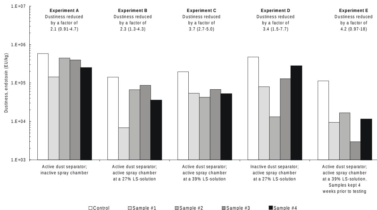
Figure 6. Dustiness of chopped straw (barley) in terms of endotoxin units (EU) emitted per unit mass (kg) of straw. Dustiness is given versus techniques to reduce the dustiness. The factor of reduction in dustiness is given with reference to the control sample, presented as the geometric mean; 95% confidence interval in parentheses.
