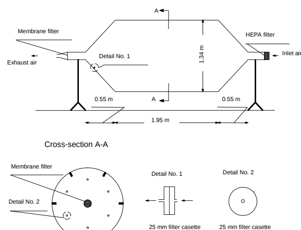
Figure 2. Rotating drum dustiness tester. The drum was operated at 7 rpm at an airflow rate of 420 l min -1 .
