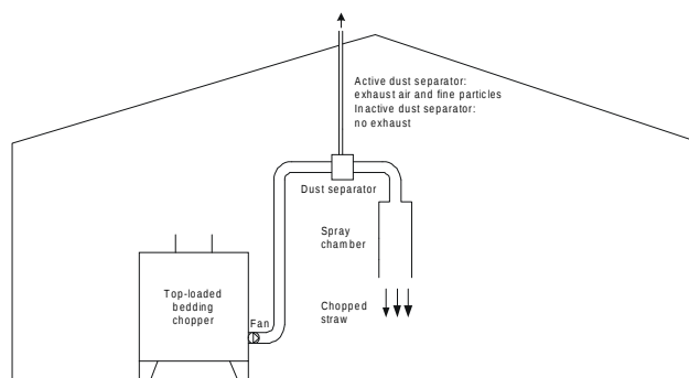
Figure 1. Experimental set-up (not to scale). The bedding chopper was fitted with a dust separator and a spray chamber.
