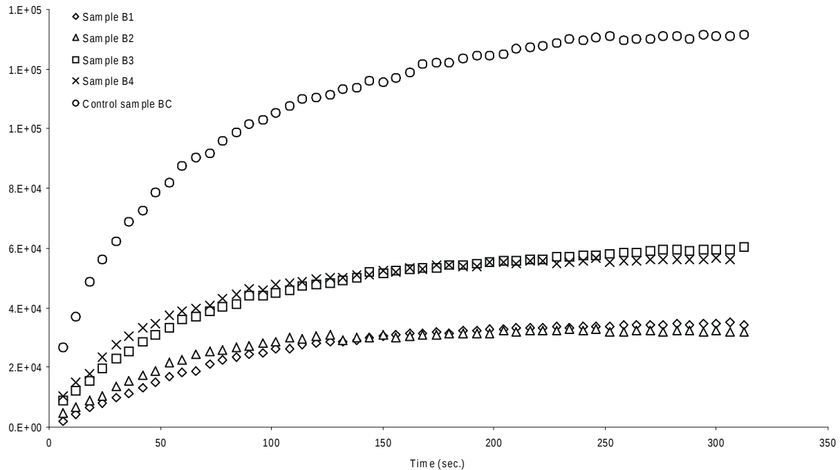
Figure 4. The concentration of airborne dust versus time after start of the rotating drum dustiness tester. Data are from experiment B.
