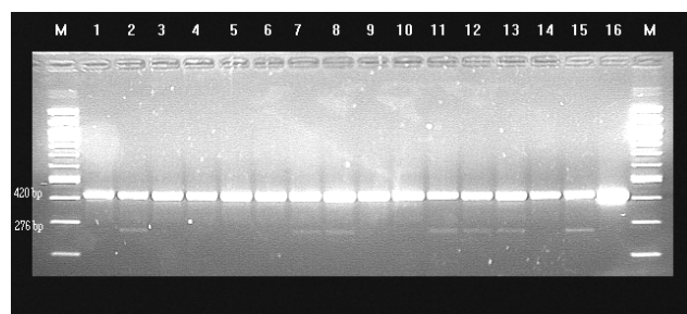
Figure 1. Agarose gel electrophoresis. Results of single-tube nested PCR amplification of flagellum gene sequence specific for Borrelia burgdorferi sensu lato (276 bp fragment). 420 bp fragment resulting from amplification of internal control (102 copies of MIMIC internal control ligated into the plasmid). Lane 1–4 sample from Ixodes ricinus , 5–13 from mosquito larvae. Lanes 5, 6, 9, 10 - negative samples, 7, 8, 11–13 positive samples. Lane 14 - isolation negative control (PCR mixture obtained an equivalent volume of distilled water instead of DNA added to the other samples), 15 - positive isolation control (isolation of 102 spirochetes), 16 - PCR negative control (distilled water instead of DNA). M - 100 bp ladder molecular weight standard. Samples in lanes 2, 7, 8, 11, 12 and 13 are positive.
